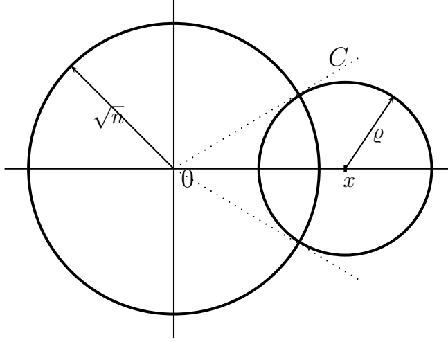
Figure 2. Concentration on S(0, \sqrt{n}) .
