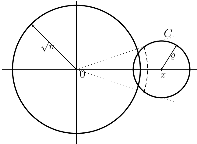
Figure 1. Concentration outside S(0, \sqrt{n}) .
