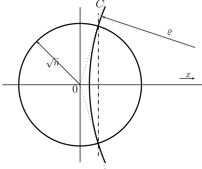
Figure 3. Concentration far from S(0, \sqrt{n}) \cap x^\perp .
